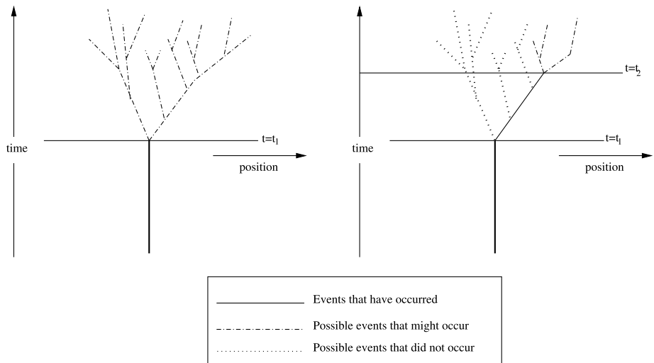
Fig. 1 Motion of a particle world line controlled in a random way, so that what happens is determined as it happens. On the left events are determined till time t_1 but not thereafter; on the right , events are determined till time t_2 > t_1 , but not thereafter
