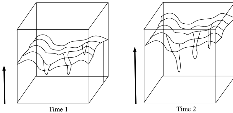
Fig. 3 An evolving curved space-time picture that takes micro-phenomena seriously. Like the EBU (Fig. 2), but here small pockets of potentiality remain unresolved till later times: delayed choice experiments can influence these ‘past’ events. The resolution of potential to definite outcomes takes place in a way like a crystallizing mixture, with pockets of residue remaining behind for a time after the main resolution front has passed
