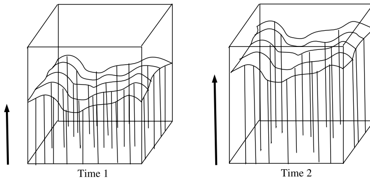
Fig. 2 An evolving curved space-time picture that takes macro-phenomena seriously. Time evolves along each world line, extending the determinate spacetime as it does so. The particular surfaces have no fundamental meaning and are there for convenience only (one requires some coordinates to describe what is happening). You cannot locally predict uniquely to either the future or the past from data on any ‘time’ surface (even though the past is already determined). This is true both for physics, and (consequently) for the spacetime itself: the developing nature of spacetime is determined by the evolution (to the future) of the matter in it
